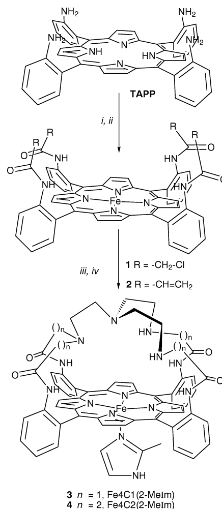
Scheme 1 Reagents and conditions: (i) chloroacetyl chloride or acryloyl chloride in dry THF-NEt 3 ; (ii) FeBr 2 -THF-2,6-lutidine under nitrogen; (iii) TREN in THF or MeOH at 55 °C; (iv) 1000 equiv. 2-methylimidazole.
